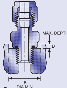
COUNTERBORED PORT
