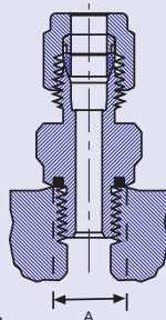
Figure 1 A DIA. MIN.
