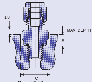
Figure 3 C DIA. MIN. MAX. DEPTH E 1/8
